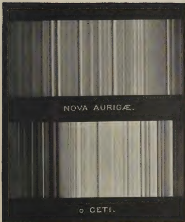
STAR SPECTRA
